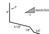
20a GAMBREL FLASHING PF11 4:12 PITCH STANDARD UNLESS SPECIFIED OTHERWISE
