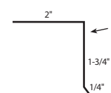
22a 2 x 2 EAVE EDGE FT03 4:12 PITCH STANDARD UNLESS SPECIFIED OTHERWISE
