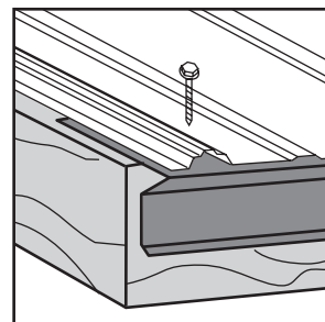
22. Drip Edge - Diverts water away from house along eave.
