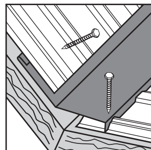
19b. Notched Transition Flashing - Profiled fit to protect against leaks at a pitch change from low to high.
